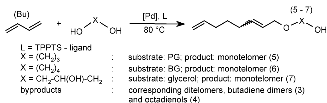
Scheme 2. Biphasic telomerization of butadiene with glycol substrates.
