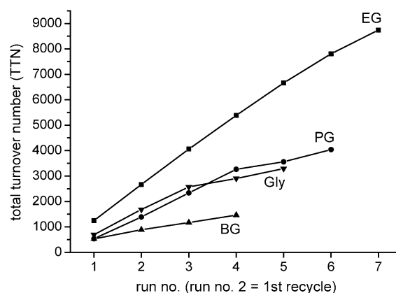
Figure 1. Overall catalyst productivities obtained during telomerization experiments with glycol substrates. Conditions: Bu/glycol = 2.5/1; cat. 0.06 mol % (based on glycol) Pd(acac) 2 + 5 equivs. TPPTS; ligand supplementation: 2.5 equivs. per recycle; 10–12 mL H 2 O; 20–30 mL glycol; 80 °C; 1200 rpm; 4 h. Substrates: EG (■), PG (●), BG (▲), Gly (▼).
