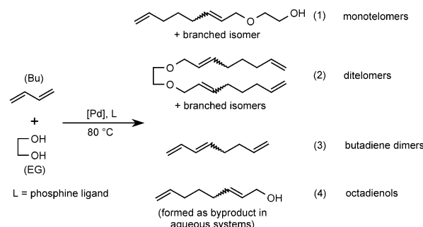
Scheme 1. Telomerization of butadiene with ethylene glycol.
